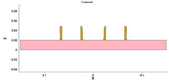
Fig. 4. Spacer geometry for an LTO deposition process and an etching process with \sigma=0.8 where the thickness of the layer deposited by CVD is reduced by 10 % compared to the process for which the result is shown in Fig. 3 (c).
